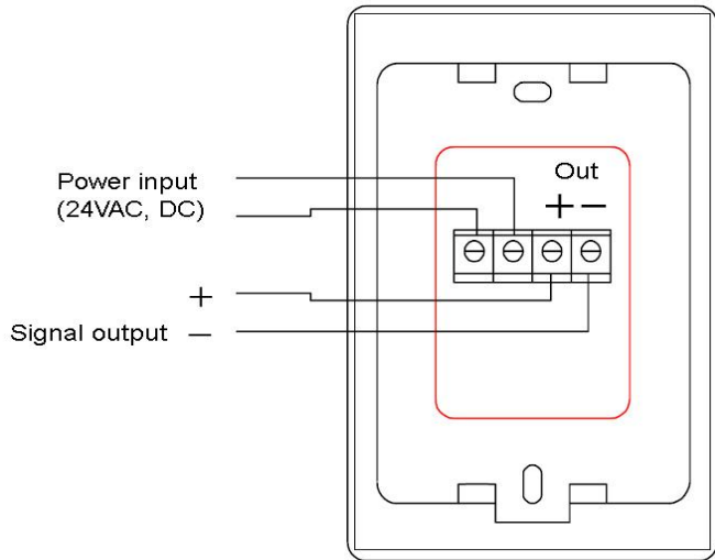
Fig. 3 CDS2000A1000 wiring
