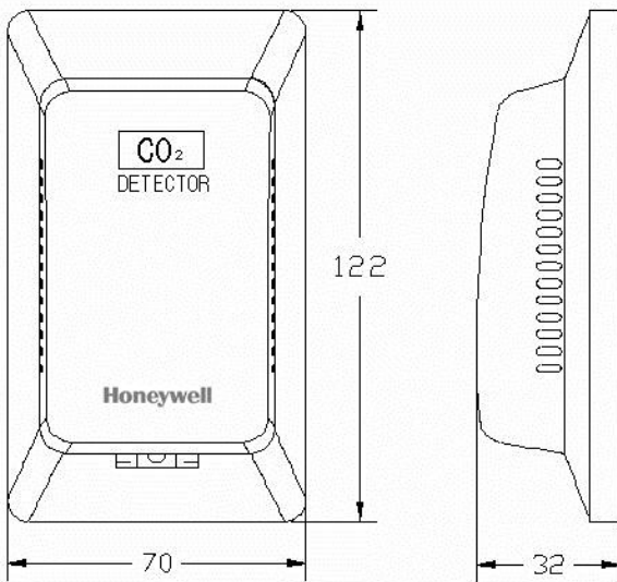
Fig. 1 CDS2000A1000 dimensions (mm)
